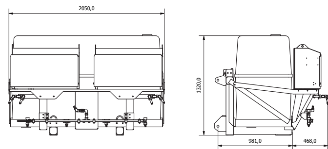
Liquid spreader CLT-1.8/2.1
